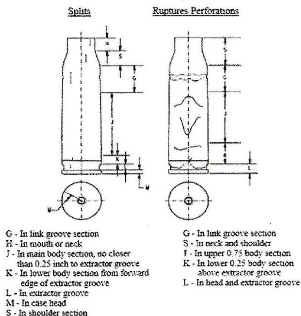
Figure 1. Identification of defects for cartridge case
