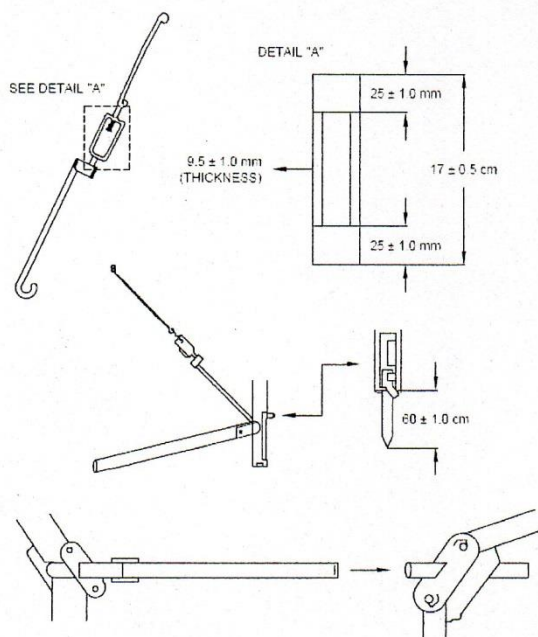
TURN BUCKLE
