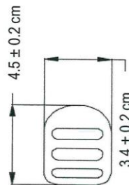
LADDER LOCK
